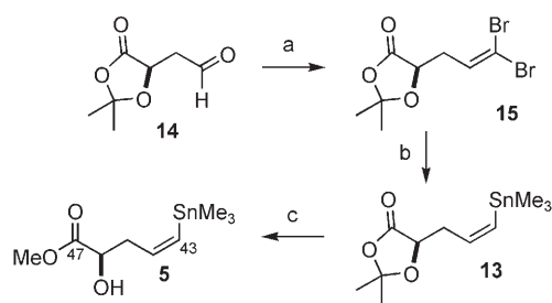
Scheme 4. Preparation of the side chain stannanes 13 and 5 . a) \text{CBr}_4 , \text{PPh}_3 , \text{Et}_3\text{N} , \text{CH}_2\text{Cl}_2 , 0^\circ\text{C} , 81%; b) n\text{Bu}_3\text{SnH} , [\text{Pd}(\text{PPh}_3)_4] , benzene, 40^\circ\text{C} ; ( \text{Me}_6\text{Sn}_2 ), i\text{Pr}_2\text{NEt} , 80^\circ\text{C} , 74%; c) \text{K}_2\text{CO}_3 , \text{MeOH} , 81%.
