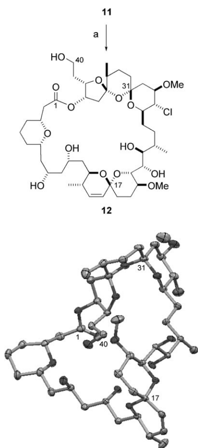
Scheme 3. Deprotection of the macrocycle 11 to the crystalline pentanol 12 and X-ray crystal structure of 12 (shown with ellipsoids at 50% probability). a) HF-Py/Py, THF, 83%.
