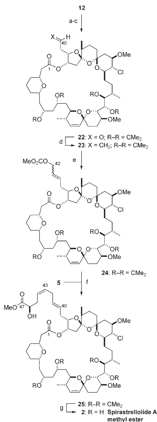
Scheme 6. Completion of the total synthesis of spirastrellolide A methyl ester ( 2 ). a) PPTS, (MeO) 2 CMe 2 /CH 2 Cl 2 (2:1), 35°C, 95%; b) PPTS, CH 2 Cl 2 /MeOH (12:1), 0°C, 78% after one recycle; c) DMP, NaHCO 3 , CH 2 Cl 2 , 80%; d) Ph 3 P=CH 2 , THF, –78°C to RT, 75%; e) 2nd generation Grubbs catalyst, 21 , benzene, 80°C, 57% (99% brsm); f) [PdCl 2 (MeCN) 2 ], 5 , DMF/H 2 O (4:1), 35°C, 96%; g) PPTS, MeOH, 35°C, 60%. PPTS = pyridinium para -toluenesulfonate.
