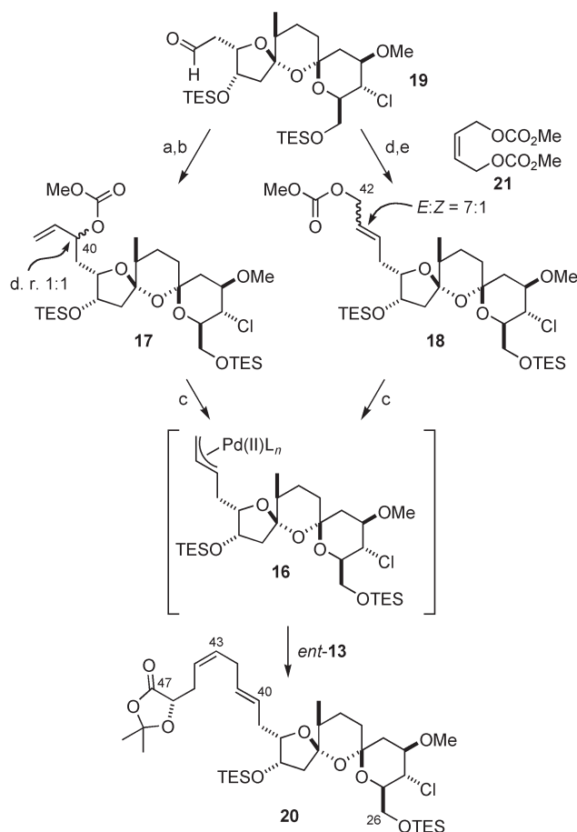
Scheme 5. Synthesis of carbonates 17 and 18 , and their coupling with stannane ent - 13 . a) \text{H}_2\text{C}=\text{CHI} , \text{CrCl}_2 , \text{NiCl}_2 , \text{DMF} , 71%; b) \text{ClCO}_2\text{Me} , \text{Py} , \text{CH}_2\text{Cl}_2 , 43%; c) [\text{PdCl}_2(\text{MeCN})_2] , ent - 13 , \text{DMF}/\text{H}_2\text{O} (4:1), 59% (for 17 ), 80% (for 18 ); d) \text{Ph}_3\text{P}=\text{CH}_2 , \text{THF} , -78^\circ\text{C} to \text{RT} , 71%; e) 2nd generation Grubbs catalyst, 21 , \text{CH}_2\text{Cl}_2 , 40^\circ\text{C} , 99% ( E/Z 7:1). \text{DMF} = N,N -dimethylformamide.
