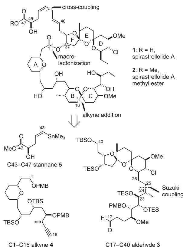
Scheme 1. Spirastrellolide A ( 1 ), its methyl ester ( 2 ), and retrosynthetic analysis leading to key building blocks 3 – 5 . PMB = para -methoxybenzyl, TBS = tert -butyldimethylsilyl, TES = triethylsilyl.
